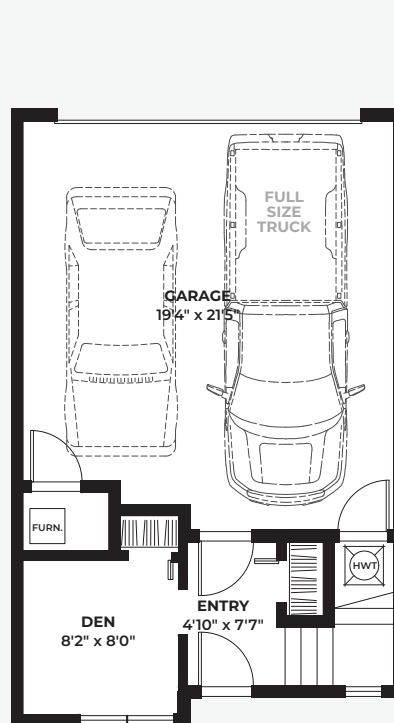
LOWER FLOOR 181 SF
