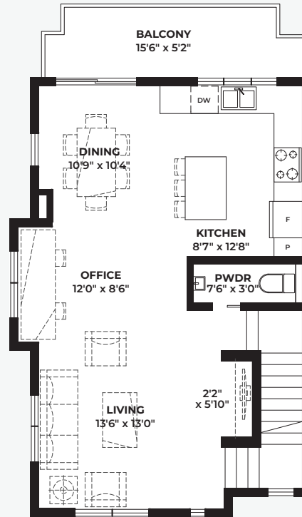
MAIN FLOOR 651 SF
